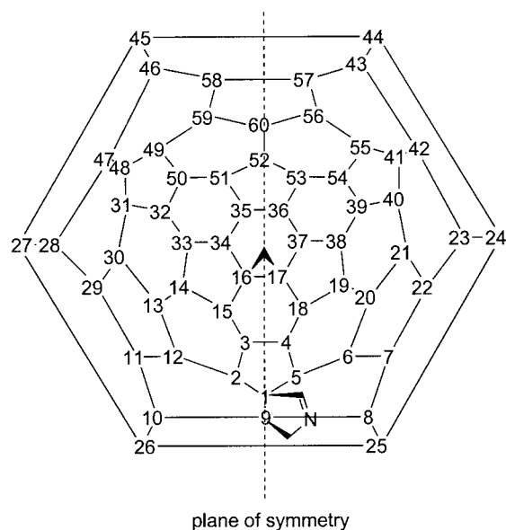
Figure 1. Schlegel diagram of bis-adduct 6 (the tether is removed for clarity).
