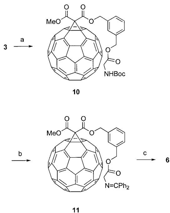
Scheme 3. Alternative synthesis of the mixed-tethered compound 6 . a) C_{60} (1 equiv.), CBR_4 (1 equiv.), DBU (2 equiv.), toluene, room temp., 18 h, 32%; b) i) TFA, DCM, 18 h, ii) benzophenone imine, THF, room temp., 62% from 10 ; c) CBR_4 (1 equiv.), DBU (2 equiv.), toluene, room temp., 1 h, 30%.
