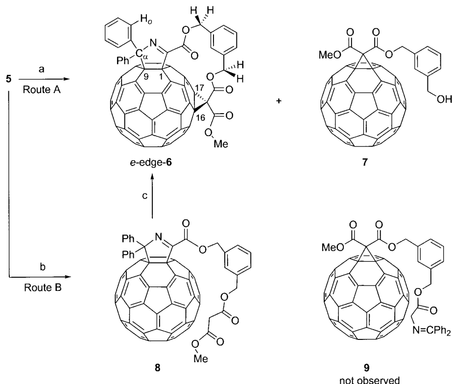
Scheme 2. Synthesis of the mono- and bis-adducts, 8 and 6 , respectively. a) C_{60} (1 equiv.), CBR_4 (2 equiv.), DBU (4 equiv.), toluene, room temp., 18 h, 30%. b) C_{60} (1 equiv.), CBR_4 (1 equiv.), DBU (2 equiv.), toluene, room temp., 2 h, 19%. c) CBR_4 (1 equiv.), DBU (2 equiv.), toluene, room temp., 18 h, 20%.
