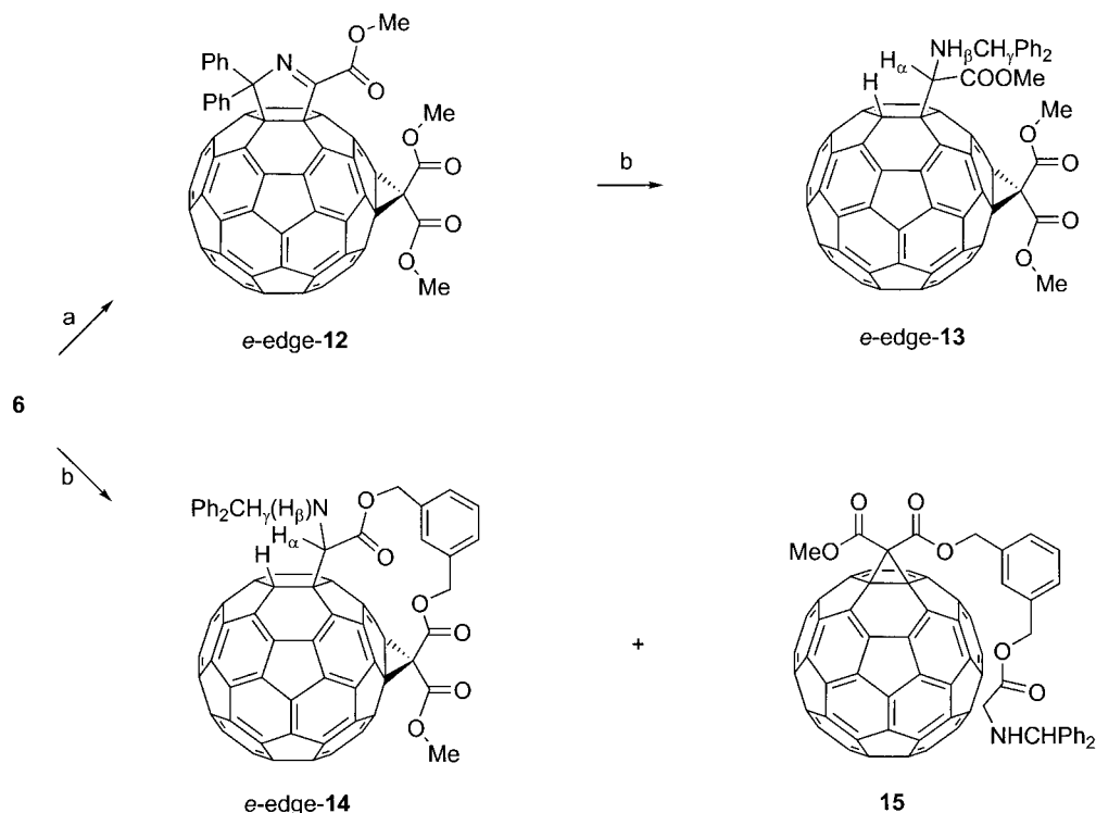
Scheme 4. Reductive ring-opening reactions of bis-adducts 6 and 12 . a) \text{K}_2\text{CO}_3 , THF/MeOH (10:1), room temp., 18 h, 40%; b) \text{BF}_3 \cdot (\text{OEt}_2)_2 , HOAc, \text{NaCNBH}_3 , DCM, room temp., 15 min, 40% from 12 , 18 h, 50% from 6 .
