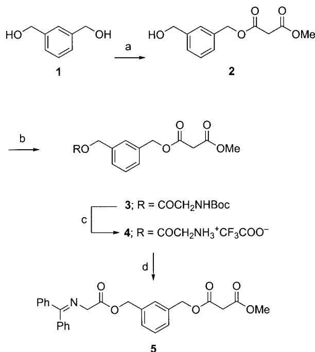
Scheme 1. Synthesis of the mixed-tethered system 5 . a) methyl malonyl chloride, triethylamine, THF, room temp., 3 h, 83%; b) N -Bocglycine, DMAP, DCC, THF, room temp., 18 h, 64%; c) TFA, room temp., 1 h, 60%; d) benzophenone imine, DCM/MeCN, room temp., 24 h, 44%.
